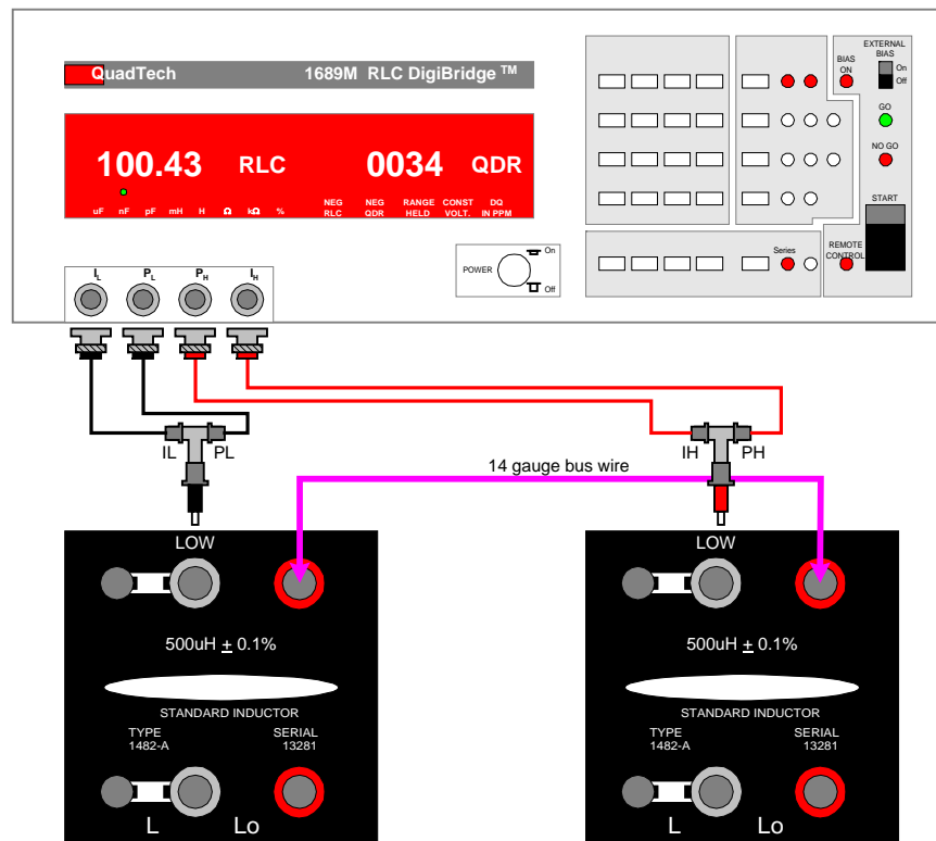
Figure 2: Connection of 1689 DigiBridge to 1482-A Inductor
